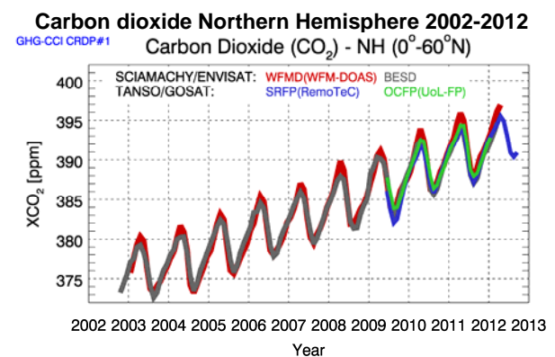
Fig. 1: Time evolution of Northern Hemispheric XCO 2 , i.e., of the column-averaged CO 2 mixing ratio, as retrieved from SCIAMACHY/ENVISAT and TANSO-FTS/GOSAT using four different GHG-CCI retrieval algorithms (see Sect. 4). Clearly visible is the CO 2 seasonal cycle - primarily caused by uptake and release of CO 2 by the terrestrial biosphere - and the atmospheric CO 2 increase with time, which is primarily caused by burning of fossil fuels. Also visible is the good agreement of the different CO 2 data products. Perfect agreement is not expected due to different spatio-temporal sampling and different altitude sensitivities (averaging kernels).
